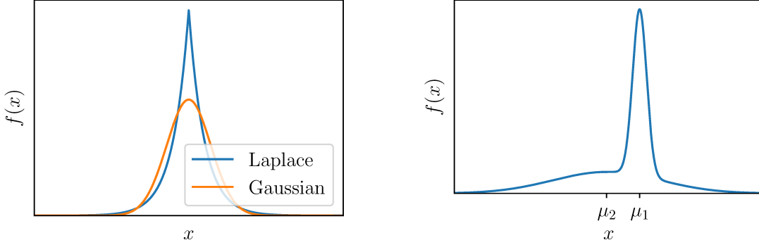
Figure 1: Example distributions
