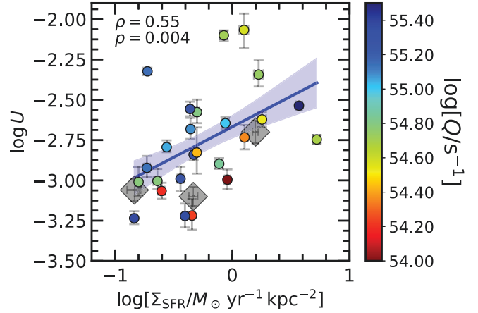
Figure 6. Relationship between \log U and \log[\Sigma_{\text{SFR}}/M_{\odot} \text{ yr}^{-1} \text{ kpc}^{-2}] for 25 individual galaxies in the MOSDEF-LRIS sample (Topping et al. 2020a) with robust size, and hence \Sigma_{\text{SFR}} , measurements (circles), and detections of \text{H}\alpha , color coded by \log[Q/\text{s}^{-1}] (see Section 5.1.1). The Spearman correlation coefficient and p -value are indicated. The solid blue line and shaded region indicate a linear fit to the data and the 1\sigma confidence interval, respectively, with the following relation: \log U = (0.379 \pm 0.030) \log \left[ \frac{\Sigma_{\text{SFR}}}{M_{\odot} \text{ yr}^{-1} \text{ kpc}^{-2}} \right] - 2.668 \pm 0.068 . Average values obtained from fitting composite spectra in three equal-number bins of \Sigma_{\text{SFR}} (from Reddy et al. 2022) are shown by the large grey diamonds.
