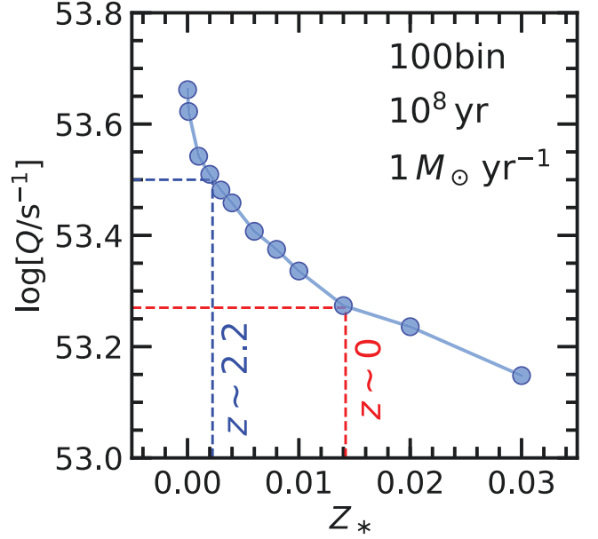
Figure 8. Q as function of Z_* for the BPASS 100bin models with an age of 10^8 yr and a constant star-formation rate of 1 M_\odot \text{ yr}^{-1} . Also indicated are the \langle Z_* \rangle inferred for z \sim 0 and z \sim 2.2 galaxies at a fixed stellar mass of \sim 10^{10} M_\odot from Kashino et al. (2022): \langle Z_* \rangle \simeq 0.0142 (roughly solar) and \langle Z_* \rangle \simeq 0.002 , respectively. The model predictions indicate \langle \log[Q/\text{s}^{-1}] \rangle \simeq 53.50 and 53.27 , respectively, for these two values of \langle Z_* \rangle .
