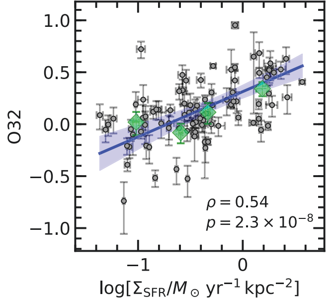
Figure 4. O32 versus \log[\Sigma_{\text{SFR}}/M_{\odot} \text{ yr}^{-1} \text{ kpc}^{-2}] for 93 galaxies in the “ionization parameter” sample with S/N \geq 3 detections of [O II], [O III], H \beta , and H \alpha (grey points). A Spearman test on the individual measurements for the 93 galaxies indicates a correlation coefficient of \rho = 0.54 , with a probability p = 2.3 \times 10^{-8} that there is a null correlation between O32 and \Sigma_{\text{SFR}} . A linear fit to the data and the 1\sigma confidence interval are indicated by the blue line and shaded region, respectively: \text{O32} = (0.415 \pm 0.064) \log[\Sigma_{\text{SFR}}/M_{\odot} \text{ yr}^{-1} \text{ kpc}^{-2}] + 0.307 \pm 0.030 . The average O32 values derived from composite spectra of galaxies in three bins of \Sigma_{\text{SFR}} are shown by the large green diamonds.
