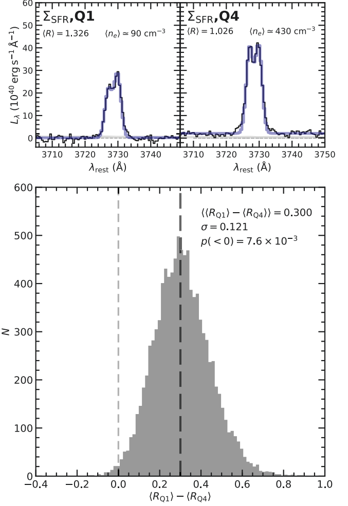
Figure 2. Top: Composite spectra of the [O II] \lambda\lambda 3727, 3730 doublet for galaxies in the lowest (left) and highest quartiles (right) of \Sigma_{\text{SFR}} . The grey shaded regions indicate the composite error spectra. Model fits to the [O II] doublet are indicated in blue, with the average line ratio, \langle R \rangle = \langle [\text{O II}] \lambda 3730 / [\text{O II}] \lambda 3727 \rangle , and inferred density, \langle n_e \rangle , indicated in each panel. Bottom: Distribution of the difference in line ratios measured from 10,000 realizations of the composite spectra in the lowest and highest quartiles of \Sigma_{\text{SFR}} . The long-dashed line indicates the average difference of \langle \langle R_{\text{Q1}} \rangle - \langle R_{\text{Q4}} \rangle \rangle = 0.300 . Also indicated are the standard deviation ( \sigma ) and the probability that the average line ratios measured for the two quartiles are equivalent.
