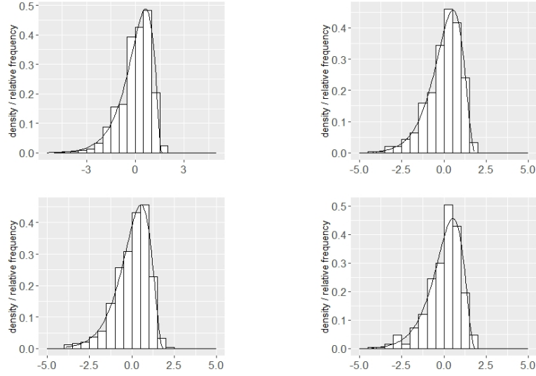
Figure 2: Histograms of \tilde{\zeta}_t^* , along with superimposed densities of negative centered and scaled \chi_k^2 distributions with df identified via K-S goodness of fit test. Top panels: p = 25 , and p = 50 , (fitted distributions with df=5, 7, respectively. p-values of K-S test: 0.90, 0.95, respectively.) Bottom panels: p = 150 and p = 250 . (fitted distributions with df=7, 8, respectively. p-values of K-S test: 0.99, 0.82, respectively.)
