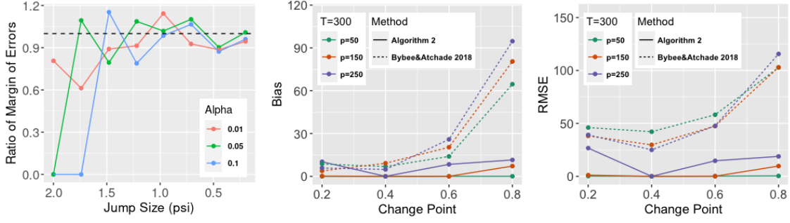
Figure 3: Left Panel: Illustration of regime adaptivity. At all considered values of \alpha = 0.1, 0.05, 0.01 , the ratio of margin of errors \left(q_{\alpha}^{nv}/(\sigma_1^{*2}\sigma_1^{-4}\psi^{-2}q_{\alpha}^v)\right) \rightarrow 1 under the non-vanishing vs vanishing regime, as the jump size \rightarrow 0 . Center and Right Panel: Comparison of estimation results (bias, RMSE) with BA 2018 at T = 300 . x-axis: change point in a fraction scale ( \tau^0/T ).
