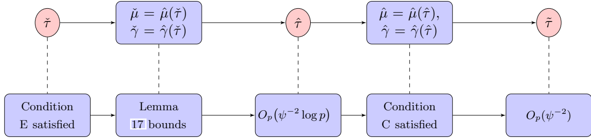
Figure 1: A schematic of the proposed Algorithm 2 and its underlying working mechanism.
