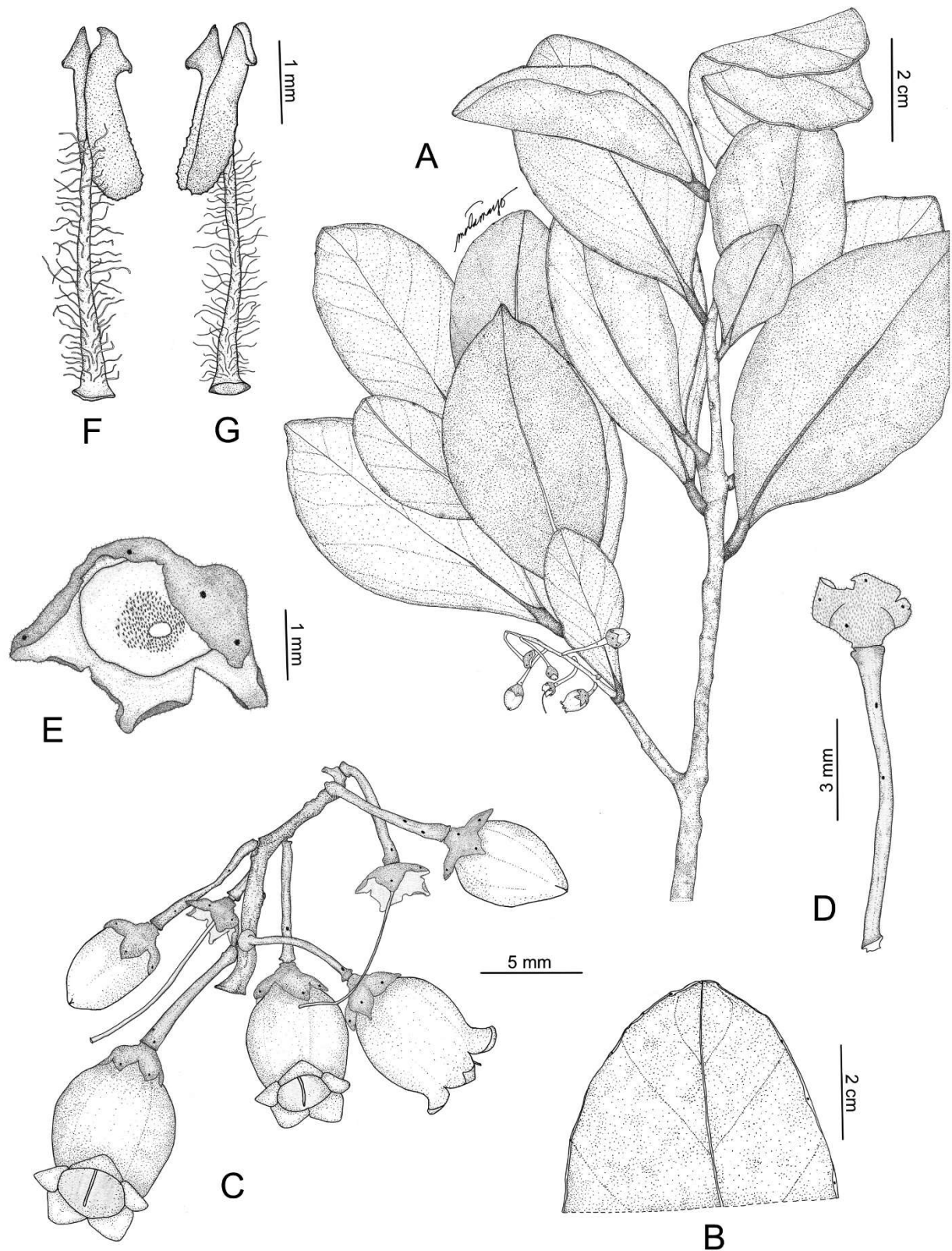
Fig. 1. Vaccinium paradoxum . A. Habit. B. Distal half of leaf showing marginal glands. C. Inflorescence. D. Pedicel and hypanthium. E. Oblique view of hypanthium showing calyx and disk. F. Dorsal view of stamen. G. Lateral view of stamen. Illustration by Maverick Tamayo. Based on the holotype.
