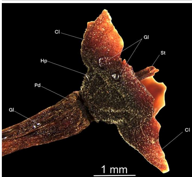
Fig. 2. Vaccinium paradoxum . Distribution of sessile glands borne on the pedicel and predominantly near the centre of the lobes. Legend: calyx lobes (Cl); glands (Gl); hypanthium (Hp); pedicel (Pd); style (St; broken). From the holotype.
