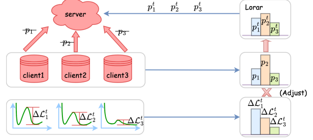
Figure 1: Our proposed re-weighting mechanism Lorar for the global model update in each round. The weight for each client (i.e., its contribution to the global model update) will be adjusted based on its loss reduction in each round. \Delta\mathcal{L}_i^t means the training loss reduction of the i -th client in the t -th round.
