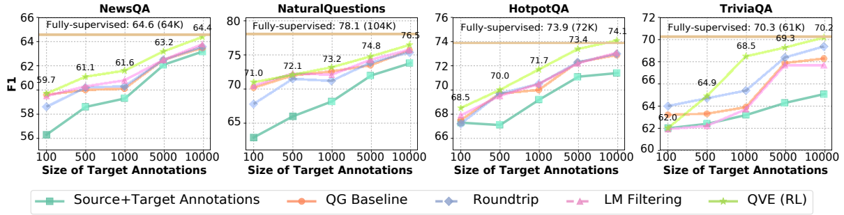
Figure 3: Impact of the number of target annotated QA pairs. We also show the fully-supervised performance (and #train) as the reference. With 10K target annotations (around 15% of the full training set), our method can achieve comparable performance to the supervised ones (as shown at the top of each sub-figure).
