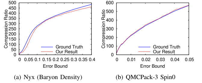
Fig. 11: Illustration of Valid Compression Ratio Range for FXRZ (using SZ)
