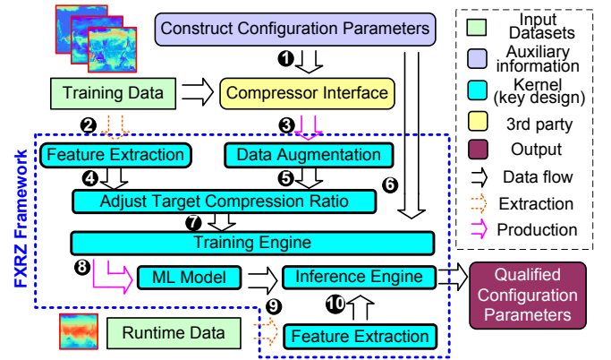
Fig. 1: Design Architecture of Feature-driven Fixed-ratio Lossy Compression Framework (FXRZ)
