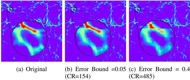
Fig. 10: Visualization of Baryon Density with Different Error Bounds (Using SZ2.1)
