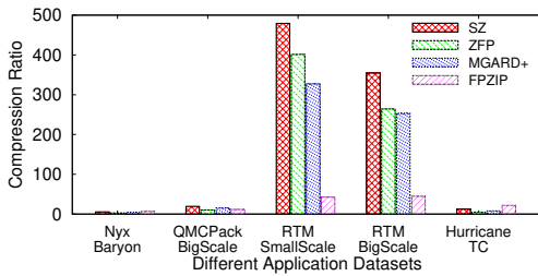
Fig. 3: Compression Ratios across Different Datasets and Compressors under an error bound.
