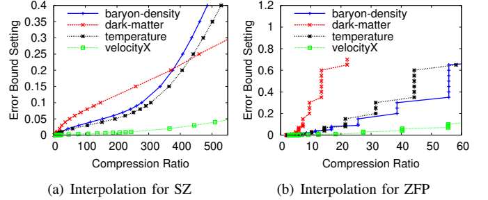
Fig. 2: Illustrating Linear Interpolation of Compression Results based on Nyx Simulation Datasets
