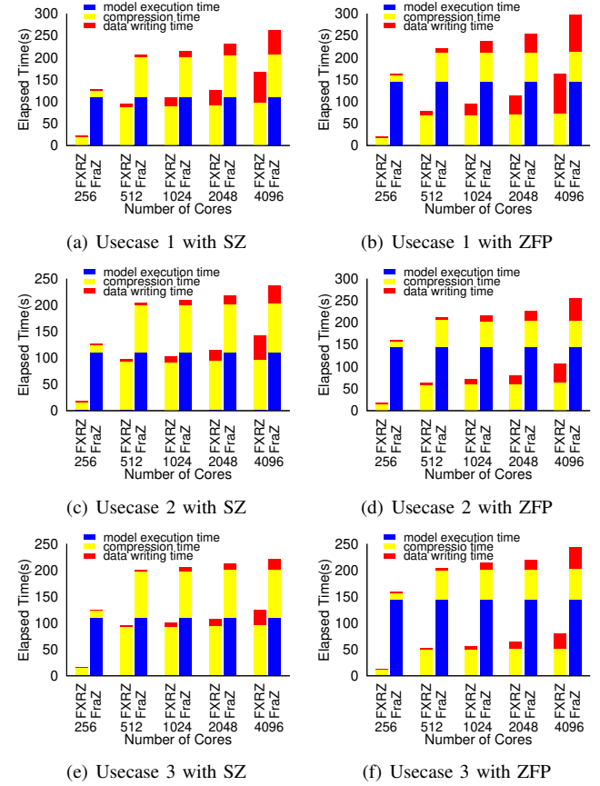
Fig. 15: Parallel Performance Evaluation (Nyx Simulation)
