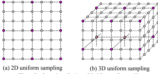
Fig. 5: 3-point Stripe Uniform Sampling
