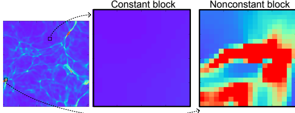
Fig. 6: Illustration of Constant/Non-constant Blocks
