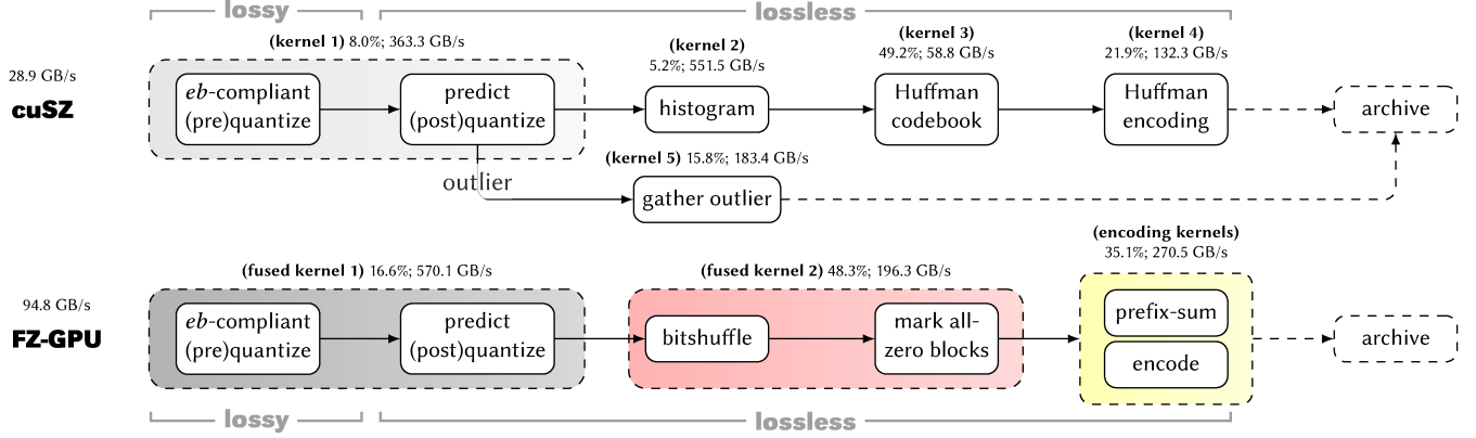
Figure 1: Our proposed new compression pipeline (“FZ-GPU”) versus original cuSZ’s compression pipeline. Each kernel is marked with number, time in percentage, and throughput (in GB/s) tested based on one field from Hurricane dataset at an error bound of 1e-4 .
