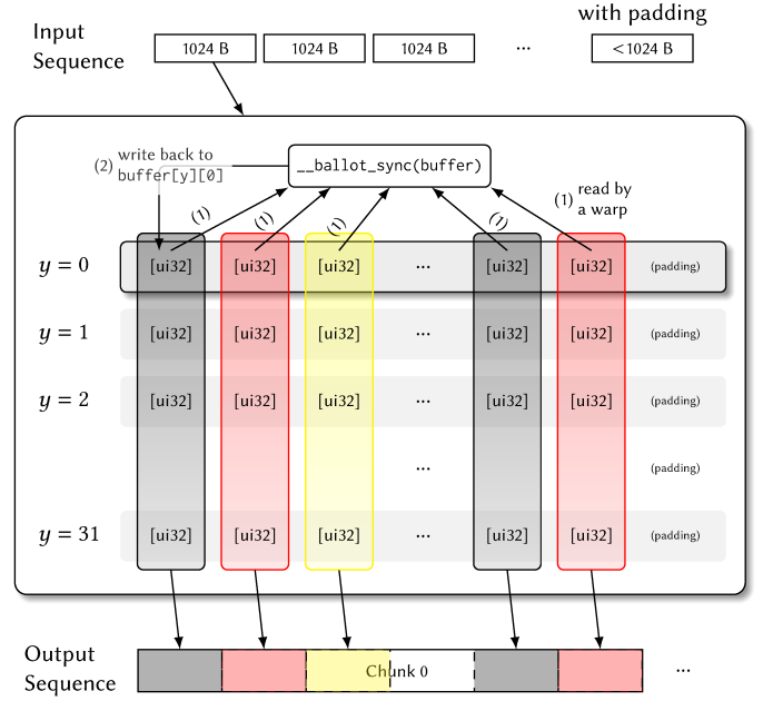
Figure 5: Our proposed scalable GPU bitshuffle method.
