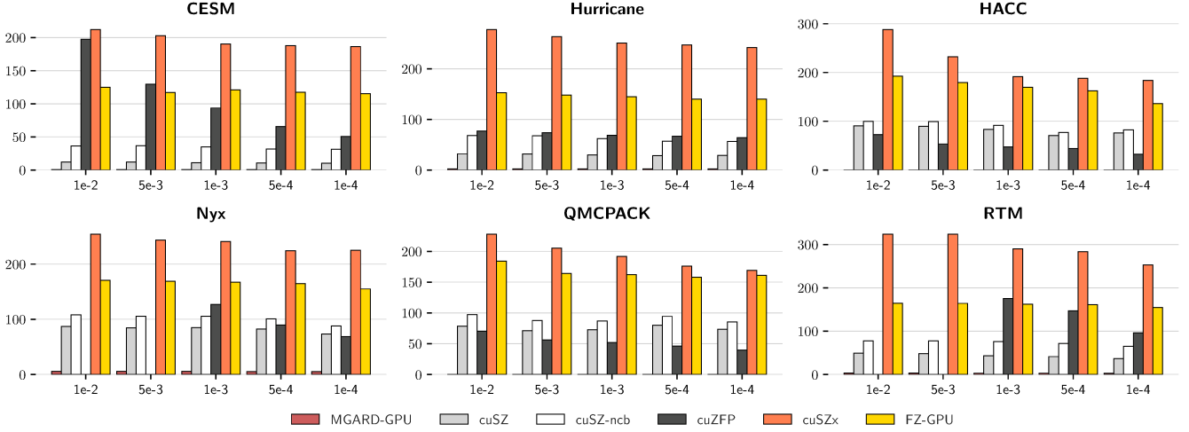
Figure 8: Compression throughput of cuZFP, cuSZ, cuSZ-ncb (cuSZ with no codebook building), cuSZx, MGARD-GPU, and FZ-GPU on NVIDIA A100. cuZFP’s throughput corresponds to FZ-GPU with the same average PSNR.
