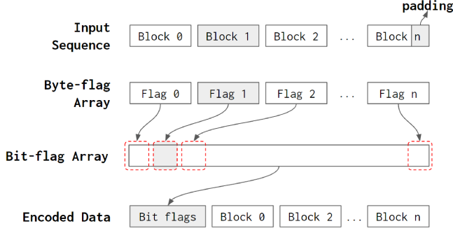
Figure 6: Our proposed fast GPU encoding method.
