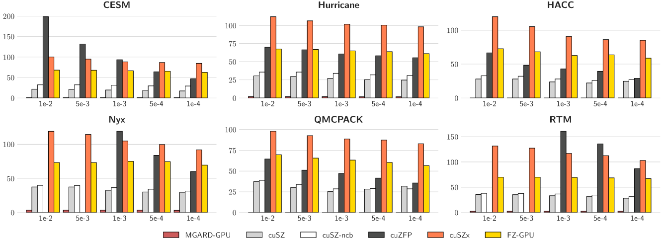
Figure 9: Compression throughput of cuZFP, cuSZ, cuSZ-ncb (cuSZ with no codebook building), cuSZx, MGARD-GPU, and FZ-GPU on NVIDIA GTX A4000. cuZFP’s throughput corresponds to FZ-GPU with the same average PSNR.
