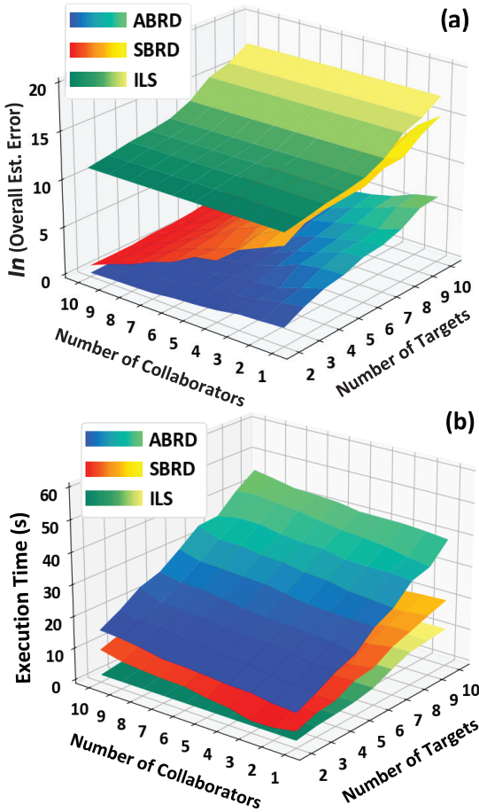
Fig. 3: Scalability analysis of the ABRD, SBRD-based symbiotic PNT solutions and the ILS algorithm.
