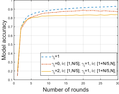
Fig. 5. Impact of model reporting coefficient on the model accuracy.
