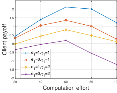
Fig. 6. Impact of clients' behavior on the payoff.
