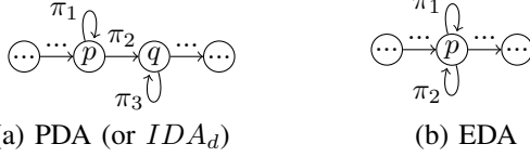
Figure 1: Illustration of Polynomial and Exponential Degree of Ambiguity (PDA, EDA) in the NFA [40]. We say that (p, \pi_2, q) is a transition from state p to state q via \text{label}(\pi_2) [20].
