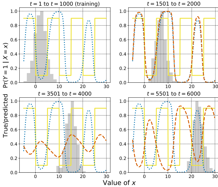
Figure 3: The adaptive behavior of Online Platt scaling (OPS) for the covariate drift dataset described in Section 1.2. The title of each panel indicates the time-window that panel corresponds to. The histogram of X_t values in the corresponding time window is plotted with maximum height normalized to 1. Also plotted is the true curve for \Pr(Y = 1 | X = x) and two predictive curves: a base model trained on t = 1 to t = 1000 , and OPS-calibrated models with parameter values fixed at the start of the time window. The base model is accurate for the training data which is mostly in [-5, 10] , but becomes inaccurate and miscalibrated with the covariate-shifted values for larger t (bottom two subplots). OPS adapts well, agreeing with the base model in the top-right subplot, but flipping the base model predictions in the bottom-right subplot.
