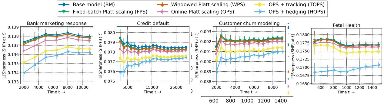
Figure 9: Sharpness results with i.i.d. data. SHP values over time of considered models on four shuffled (ie, nearly i.i.d.) datasets (Section 4.1). The drop in expected sharpness is less than 0.005 in all cases except for the HOPS forecaster on the Fetal Health dataset, where it is 0.01.
