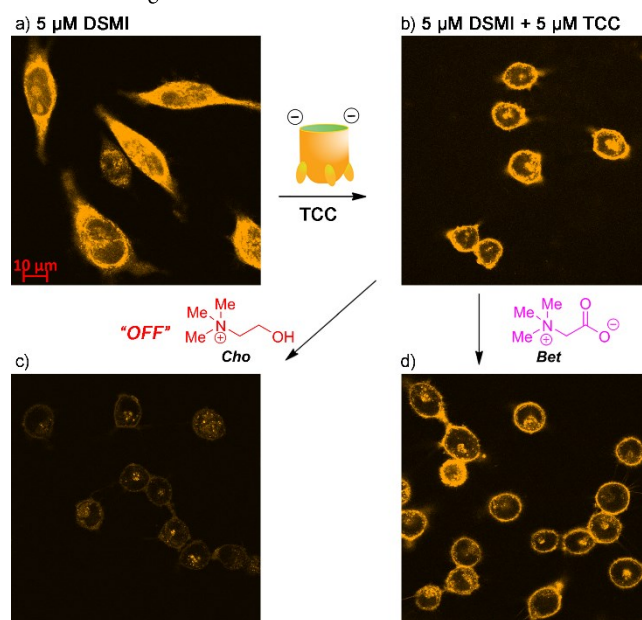
Figure 5. IDA sensing with TCC•DSMI. DSMI channel fluorescence images of live HeLa cells treated by a) 5 \mu\text{M} DSMI for 1 h; b) TCC•DSMI (pre-mix, 5 \mu\text{M} each) then PBS for 1 h; c) TCC•DSMI (pre-mix, 5 \mu\text{M} each) then 50 mM Choline for 1 h; d) TCC•DSMI (pre-mix, 5 \mu\text{M} each) then 50 mM Betaine for 1 h.
