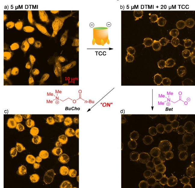
Figure 4. IDA sensing with TCC•DTMI. DTMI channel fluorescence images of live HeLa cells treated by a) 5 \mu\text{M} DTMI, b) TCC•DTMI (pre-mix, 20 \mu\text{M} , 5 \mu\text{M} ); c) TCC•DTMI (pre-mix, 20 \mu\text{M} , 5 \mu\text{M} ) + 50 mM Butyrylcholine; d) TCC•DTMI (pre-mix, 20 \mu\text{M} , 5 \mu\text{M} ) + 50 mM Betaine. Incubation time = 1 h. Image a) was captured under a lower Gain = 700.0, images b), c), d) were captured under Gain = 800.0 and larger pinhole.
