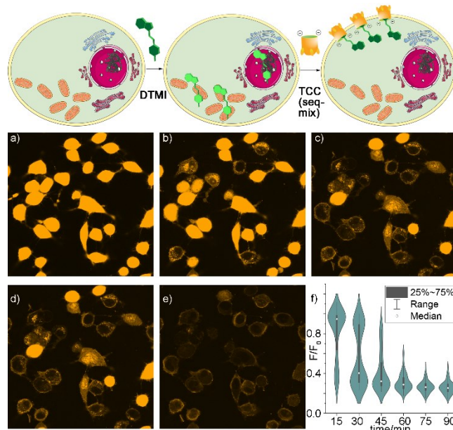
Figure 3. Intracellular Relocation. Confocal fluorescence images of live HeLa cells treated by 5 \mu M DTMI for 1 h, followed by incubation with 20 \mu M TCC (seq-mix) for a-e) 0, 15, 30, 45, and 75 mins. f) Violin plot of the integrated density ( F ) change over time measured on each
