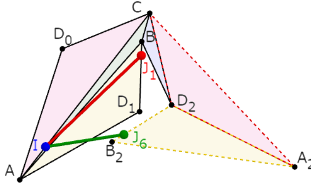
Fig. 16: A case of f_6 < 0 if p > 0 is infinitesimally close to 0.
