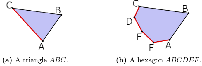
Fig. 22: Polygons that have FGG paths.
