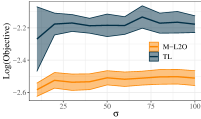
Figure 4: Performance on LASSO optimizers. We vary the standard deviation of the distribution used for sampling the weight matrix \mathbf{A} for adaptation optimizers. We visualize both the mean and the confidence interval in the figure.
