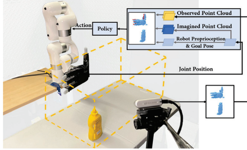
Figure 2: Real-experiment Setup: we use an Allegro Hand attached on an XArm6 and a RealSense D435 camera facing forward the robot.
