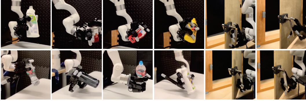
Figure 5: Real-experiment: We evaluate our point cloud policy on various unseen objects.
