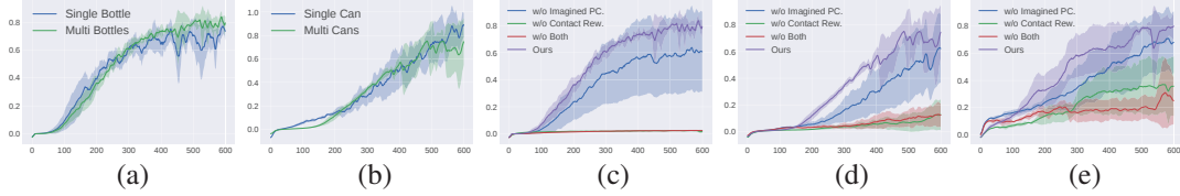
Figure 4: Training Curves. The left two plots show the single-object and multi-object training curve of (a) bottle category and (b) can category. The right three plots show the ablation results on the (c) grasping bottle (d) grasping can and (e) door opening. The x-axis is the training iterations and y-axis is the normalized episodic return. The shaded area indicates standard error and the performance is evaluated on five random seeds.
