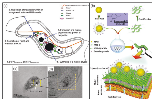
Fig. 4 Magnetotactic bacteria actuators. (a) Model of the iron reaction pathway for the bio-mineralization of the magnetosomes and its chain assembly. Adapted with Permission. 90 Copyright 2008 ACS. (b) Process of embedding iron oxide particles onto the surface of magnetotactic bacteria to enhance the actuator's magnetic response. Adapted with Permission. 78 Copyright 2019, Wiley. (c) TEM images of modified E. coli (cultured with iron) expressing mineralized mCherry-ferritin. (d) A zoomed-in image of the ferritin formed in the cytosol of modified E. coli . Adapted with Permission. 91 Copyright 2020, ACS.
