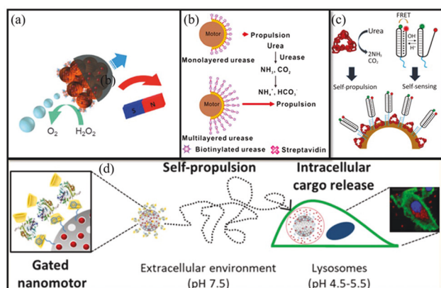
Fig. 6 Enzyme-powered actuators; (a) A magnetically bio-catalytic Janus motor coated with catalase. Adapted with Permission. 32 Copyright 2015, RSC. (b) Schematic illustration of a Janus Au/magnetic microparticles (MMPs) micromotor with multilayers of biotinylated ureases. Adapted with Permission. 110 Copyright 2020, ACS. (c) Enzyme-powered micromotors functionalized with a FRET-labelled triplex DNA nano-switch for pH sensing. Adapted with Permission. 107 Copyright 2018, ACS. (d) Schematic diagram of enzyme-powered mesoporous silica nanomotors' intracellular payload delivery. Adapted with Permission. 108 Copyright 2019, ACS.
