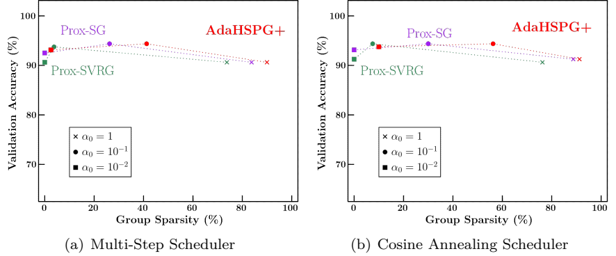
Figure 3: Validation accuracy versus group sparsity under varying step sizes.
