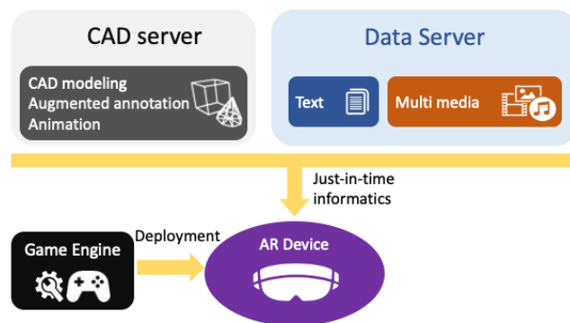
Figure 3: The system architecture fundamentally changes the role of the game engine. The software developed using the game engine retrieves the contents from the servers before presenting to users.
