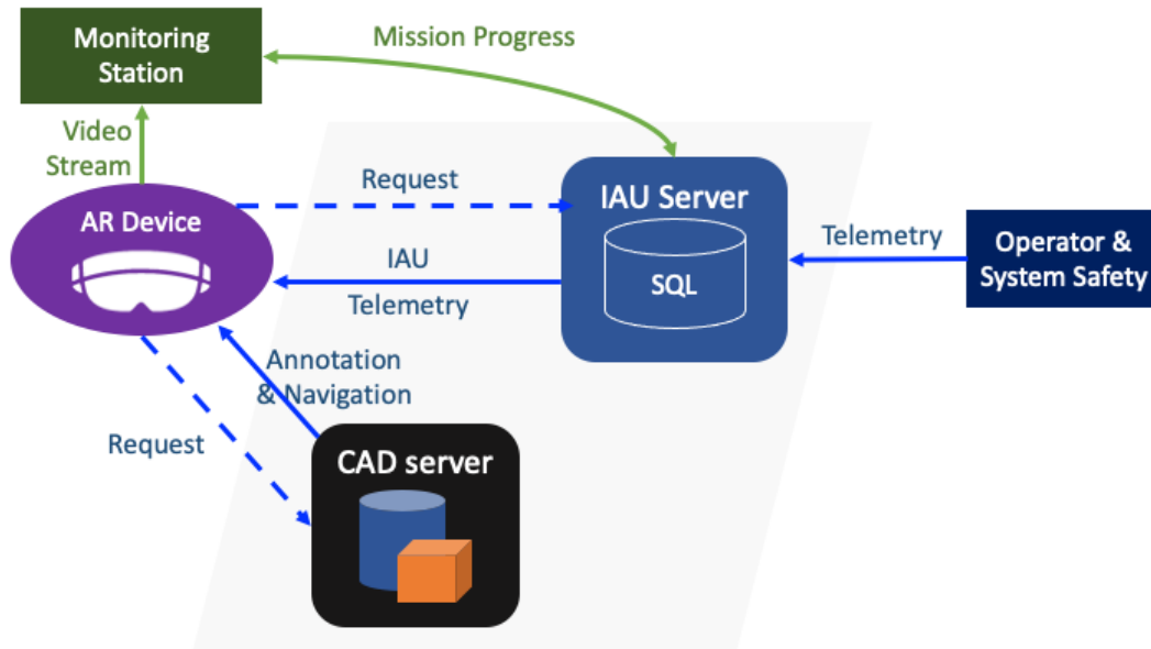
Figure 2: The underlying system architecture of the AR Systems Framework includes multiple servers. This architecture enables AR content to be disentangled from the software that presents the content to users.
