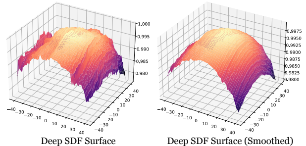
Figure 8. Visualization of DeepSDF Surface Normals within a 1.6\text{ cm} \times 1.6\text{ cm} area. From the visualization, we can clearly see an improvement in surface smoothness at a small scale, which is beneficial to the differentiable rendering process. The X-Y plane (horizontal) indicates the location on a surface with a step size of 0.2mm. Given the unit surface normal vector at a point on the grid (x, y) , we compute its dot product with the unit surface normal vector at (0, 0) , and plot this value on the Z-axis. This shows the curvature of the surface as well as its level of smoothness.
