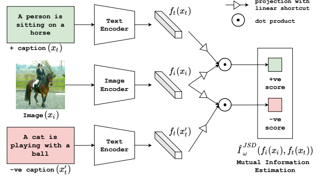
Figure 2: CLIP-Lite : We extract representations for an image, its positive caption, and one negative caption. Image-caption pairs are then fed into the mutual information discriminator function which outputs a score for each pair. These scores are then used to estimate and maximize mutual information using Jensen-Shannon Divergence (JSD) to optimize the parameters of the encoders and the mutual information discriminator end-to-end. The projection and dot function represents the MI discriminator function T_\omega .
