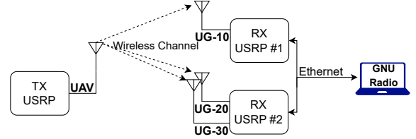
Fig. 2: Measurement system setup
