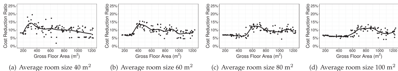
Fig. 5. Cost reduction ratio with respect to average room size and gross floor area.
