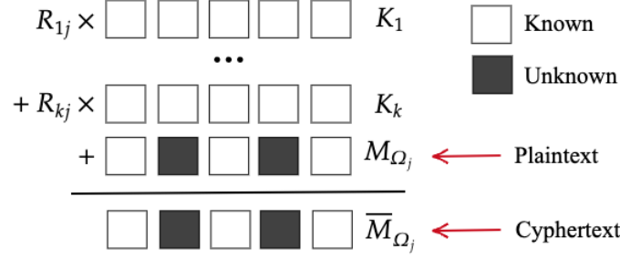
Figure 2: Our encryption method. Plaintext and cyphertext have the same set \Omega of missing entries.
