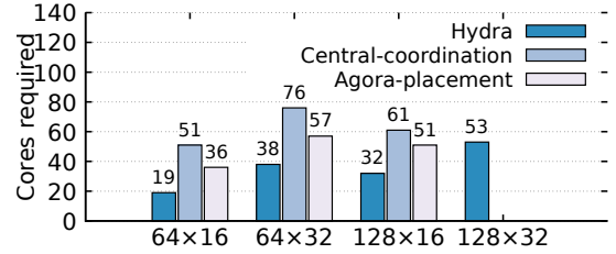
Figure 10: CPU cores needed by Hydra, Central-Coordination, and Agora-Placement for different massive MIMO dimensions (uplink).
