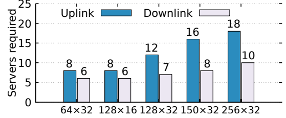
Figure 6: Number of servers required to support different massive MIMO settings in the CloudLab cluster.
