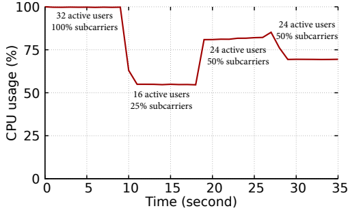
Figure 11: Hydra’s CPU usage with a dynamic workload.
