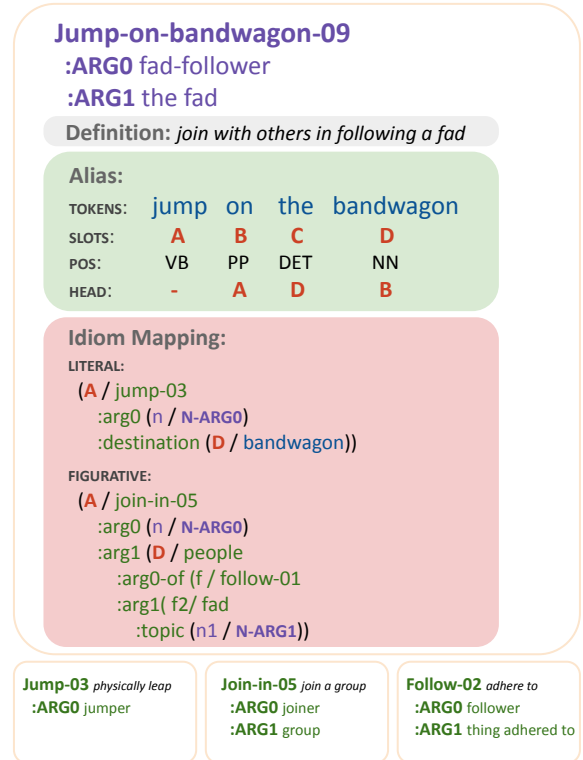
Figure 1: Roleset for jump-on-bandwagon-09 with token breakdowns and mappings between literal and figurative frames.
