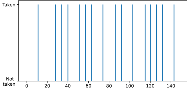
Figure 6: Prime+Probe result.
