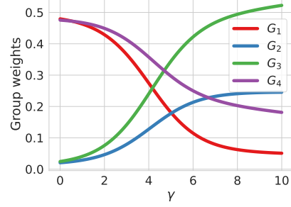
Figure 2: AFR weights on Waterbirds. Group aggregated weights as a function of \gamma on \mathcal{D}_{RW} for the Waterbirds dataset, with majority groups G_1 and G_4 , and minority groups G_2 and G_3 . The ERM model performs poorly on minority groups G_2 and G_3 , enabling automatic group rebalancing by upweighting poorly predicted examples. The reweighted group distribution is more balanced than the original group distribution, for a broad range of \gamma values.
