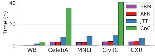
Figure 3: Training time. Training time (in hours) across different spurious correlation benchmarks. AFR only incurs a negligible overhead compared to standard ERM and is substantially less expensive than JTT and CNC.
