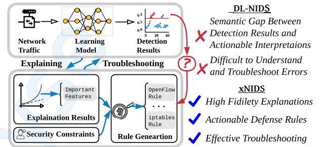
Figure 1: An illustration of how xNIDS explains DL-NIDS and enables active intrusion response.
