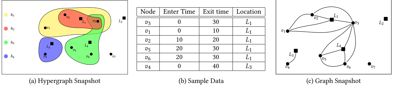
Figure 1: Sample Trace Data and their corresponding Hypergraph and Graph representations
