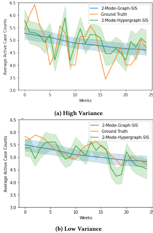
Figure 2: Plots comparing 100 runs of the best calibrated HETEROGENEOUS-GRAPH-SIS, HETEROGENEOUS-HYPERGRAPH-SIS against the ground truth average active case counts
