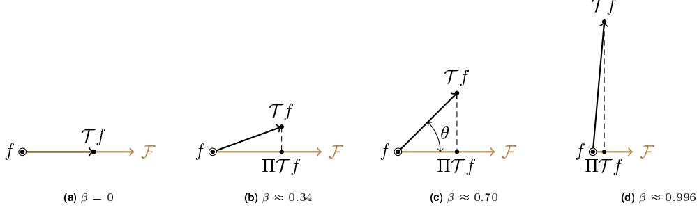
Figure 4: Local alignments between the Bellman backup \mathcal{T}f and the class \mathcal{F} for various values of \beta . The setting in Figure 4a is traditionally called ‘Bellman complete’. In this simple example \beta = \sin \theta .
