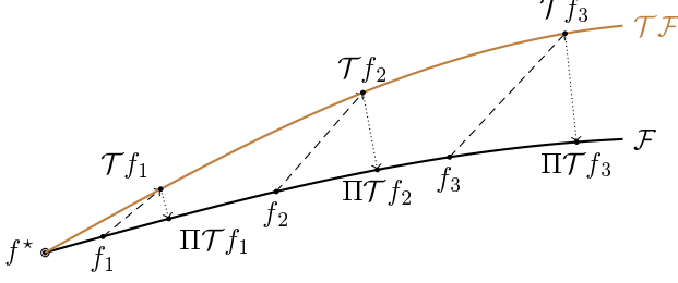
Figure 2: Local inherent Bellman errors. The norm of the un-captured component of the Bellman error \Pi T f - T f , when maximized over f \in \mathcal{F} , is the inherent Bellman error. For every function f \in \mathcal{F} , such un-captured component is always a fraction of the Bellman error f - T f . When the Bellman error is reduced, its un-captured component also gets reduced. This means that the ‘effective’ inherent Bellman error seen by an algorithm decreases as the algorithm approaches the optimal predictor f^* along \mathcal{F} . In order to leverage this observation in the analysis, we localize the inherent Bellman error to a subset of functions where the empirical predictor \hat{f} returned by the minimax algorithm is expected to be. In this way, we can replace the inherent Bellman error in Equation (8), which is defined globally over \mathcal{F} , with a more localized version defined over a smaller class \tilde{\mathcal{F}} \subset \mathcal{F} that contains \hat{f} .
