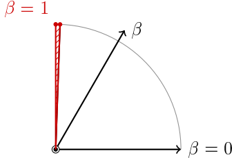
Figure 5: Off-policy reinforcement learning remains viable for values of \beta in the range [0, 1) , while prior analyses expected an unavoidable inherent Bellman error to arise. The red shaded area, which corresponds to \beta \rightarrow 1 , represents problems where the sample complexity becomes unmanageably large, a condition in force in the lower bounds.
