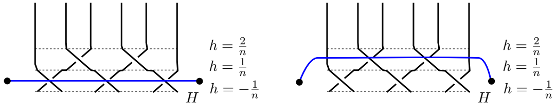
FIGURE 24. The horizontal regions containing the crossings, the horizontal line H (in blue) and the isotopies are shown for C_n^u and C_{n-1}^u .
