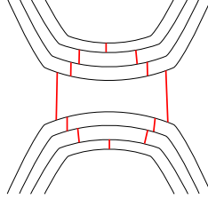
FIGURE 25. The red edges correspond to the crossings in C'_\sigma .
