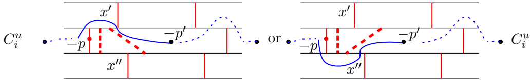
FIGURE 28. The point -p is marked with a red dot and the point -p' is marked with a black dot.
