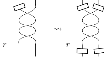
FIGURE 11. Framing the negative twist region with r = -3 .
