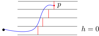
FIGURE 31. There are no other intersections of the blue arc with x_\sigma^n other than those shown because the initial construction of C'_\sigma requires that each pair in u' are the furthestest possible, one of the conditions marked by * .
