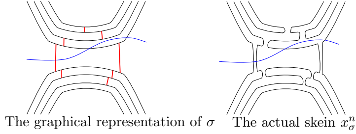
FIGURE 22. The picture shows an example of how one can recover the skein resulting from the application of a Kauffman state \sigma from a representation of black arcs and red edges. Note how the intersection of the blue arc with the red edge counts as two intersections of the blue arc with the skein x_\sigma^n .
