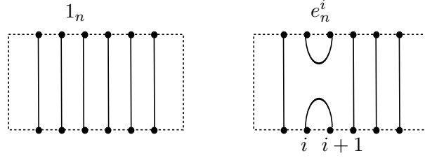
FIGURE 6. An example of the identity element 1_n and a generator e_n^i of TL_n for n = 6 and i = 2 .
