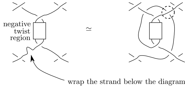
FIGURE 5. Local isotopy that turns a near-alternating diagram (left) into an almost alternating diagram (right). The single crossing change to be made in the resulting diagram to make it alternating is in the dashed circle on the right. The two diagrams agree everywhere except for the portion shown.
