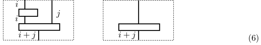
FIGURE 8. The larger projector absorbs the smaller one.
