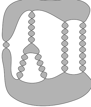
FIGURE 4. The surface S_\sigma(D) .
