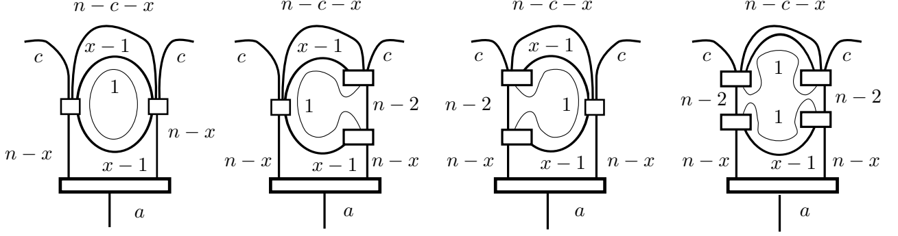
FIGURE 15. If x = k + 1 , expand and then apply the induction hypothesis to the first 3 figures.
