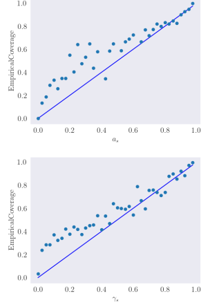
Figure 2: Assessment of posterior calibration for detection and continuous parameters, respectively shown in the graph and table. The blue lines in the graphs represent the ideal calibrations. Bayes credible intervals were constructed for 90% coverage.
