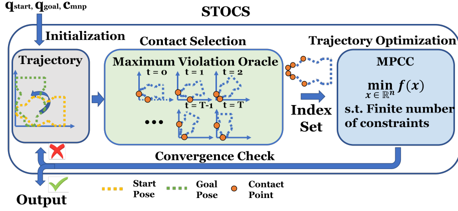
Fig. 4: Illustrating the workflow of STOCS. Given the start pose q_{start} , goal pose q_{goal} , and a manipulator contact state c_{mnp} , STOCS iterates between using the Maximum Violation Oracle to instantiate contact points, and solving a finite dimensional MPCC to decide a step direction until the convergence criteria is met. STOCS does not need a predefined contact set and can select the contact points simultaneously while solving trajectory optimization. [Best viewed in color.]
