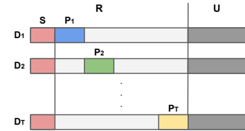
Figure 2: Illustration of the features in our data distributions.
