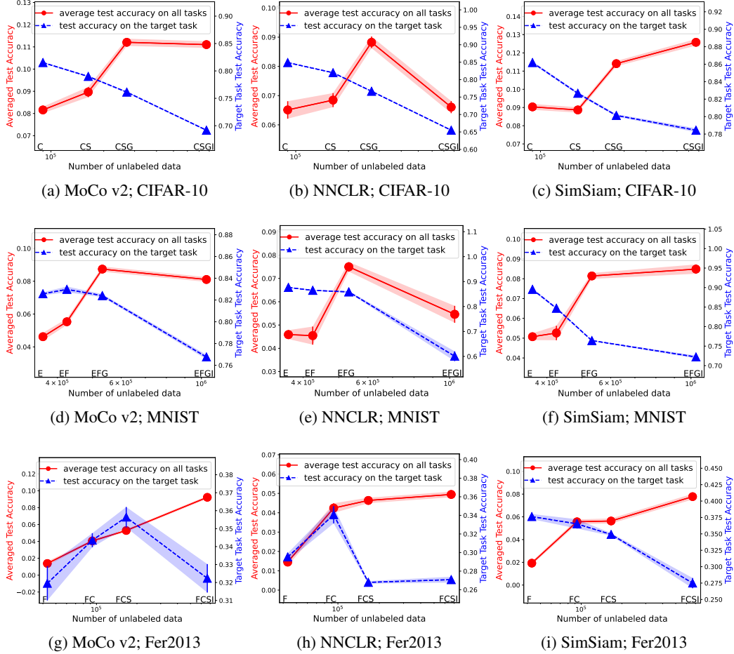
Figure 14: Trade-off of universality and label efficiency for MoCo v2, NNCLR, SimSiam on downstream tasks CIFAR-10, MNIST, Fer2013. x -axis: incrementally add datasets for pre-training. Pre-training data: (a)(b)(c) CINIC-10 (C), SVHN (S), GTSRB (G), and ImageNet32 (I). For example, “CS” on the x -axis means CINIC-10+SVHN. Target task: CIFAR-10. Red line: average test accuracy of Linear Probing on all 4 datasets. Blue line: test accuracy on the target task. (d)(e)(f) EMNIST-Digits&Letters (E), Fashion-MNIST (F), GTSRB (G), ImageNet32 (I). Target: MNIST. (g)(h)(i) FaceScrub (F), CIFAR-10 (C), SVHN (S), ImageNet32 (I). Target: Fer2013. All evaluations are trained with 1% labeled data.
