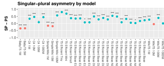
Figure 4: Singular-plural asymmetry by model for the two-noun conditions. Stars indicate significance obtained from \chi^2 tests comparing accuracy across the two conditions with Bonferroni-corrected \alpha .
