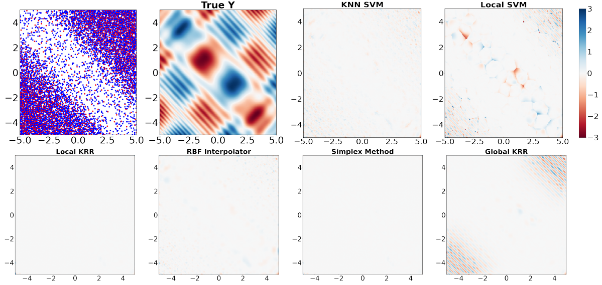
Figure 2: Synthetic data. First line, L→R: input data, true model, then prediction errors on knn-svm, local-svm. Second line, L→R: prediction errors on local KRR, RBF-Interpolator, simplex, global KRR.
