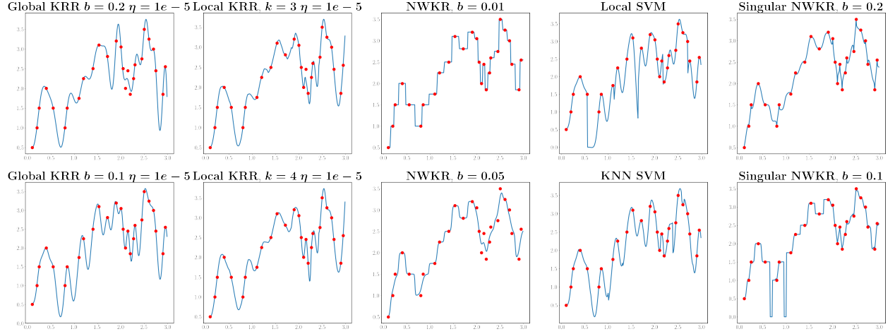
Figure 1: Fit models on synthetic data in d = 1 .
