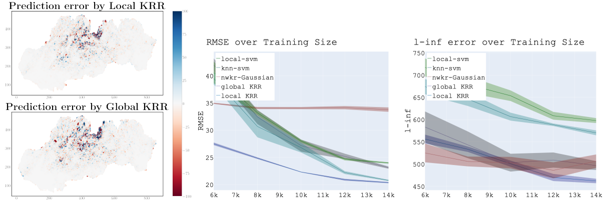
Figure 3: L→R: Prediction error, RMSE, and \ell_\infty error for Slovakian Percipitation
