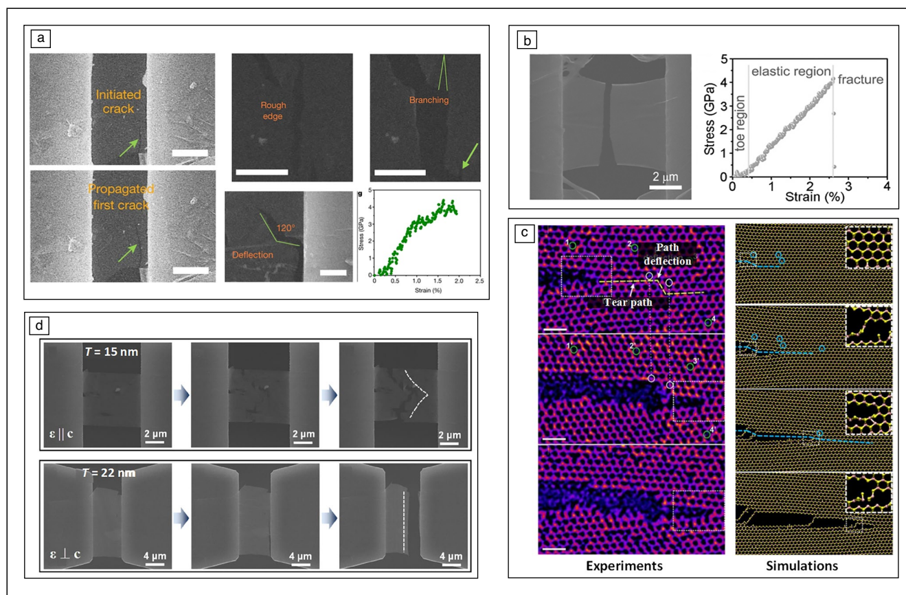
Figure 3. Experimental studies of fracture in other 2D materials beyond graphene. (a) Single-crystal monolayer h-BN that showed intrinsic toughening. Scanning electron microscope (SEM) images of the sample in the push-to-pull device, fracture edges, and the toughening mechanisms and the stress-strain response of h-BN. 36 (b) Brittle fracture of \text{MoSe}_2 SEM image and the stress-strain curve. 37 (c) Aberration-corrected transmission electron microscope images of crack propagation over time in monolayer \text{MoS}_2 with simulations modeling the observed behavior. 38 (d) SEM images of the anisotropic fracture behavior of 2D selenium. In the top figures the strength is higher and the failure strain is lower due to tension along the strong covalent bonds of 2D selenium, whereas in the lower figures the strength is lower and the failure strain is higher due to tension along the weak van der Waals bonds. 39 Scale bars: (a): 2 \mu\text{m} , (c): 1 \text{ nm} .
