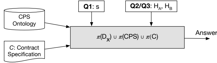
Fig. 1. Overview of Components used in Answering Queries Q1-Q3 for Agent X \in \{A, B\}
