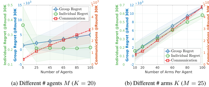
Figure 4: The performance of UCB-TCOM with different number of agents and arms
