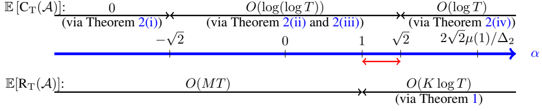
Figure 2: Impact of parameter \alpha on UCB-TCOM’s communication time \mathbb{E} [C_T(\mathcal{A})] and group regret \mathbb{E}[R_T(\mathcal{A})] . When \alpha \in (1, \sqrt{2}) , UCB-TCOM achieves the near-optimal group and individual regret upper bounds with O(\log(\log T)) communications.
