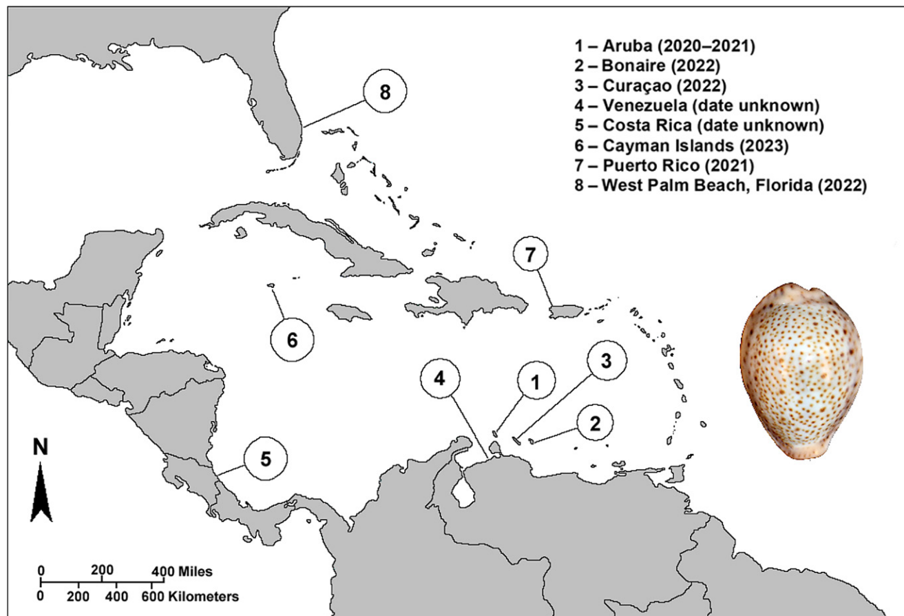
Figure 1. Known distribution of Naria turdus in the Western Atlantic and the year it was recorded in each locality.
