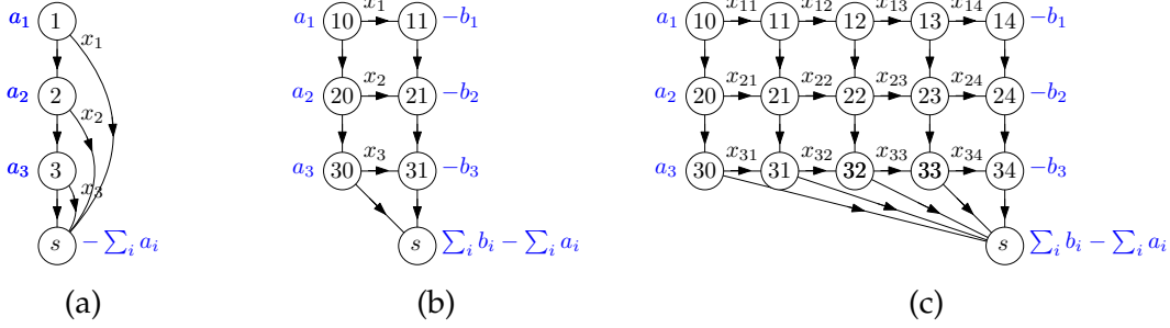
Figure 1: The first graph realizes \text{PS}_n^1(\mathbf{a}, \mathbf{0}) for n = 3 as shown by Baldoni and Vergne [1]. The second and third graphs are G(n, 1) and G(n, m) which realize as flow polytopes the original and generalized Pitman–Stanley polytopes \text{PS}_n^1(\mathbf{a}, \mathbf{b}) and \text{PS}_n^m(\mathbf{a}, \mathbf{b}) , respectively, for n = 3 , m = 1 and n = 3 , m = 4 , respectively.
