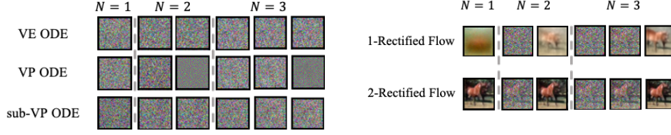
Figure 10: Few-step generation with different ODEs. Compared with VE, VP, sub-VP ODE, 1-rectified flow can generate blurry images using only 1, 2, 3 steps. After one time of rectification, 2-rectified flow can generate clear images with 1, 2, 3 steps.
