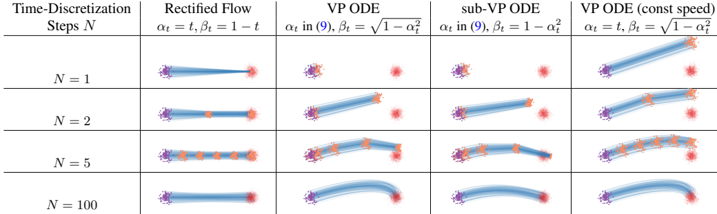
Figure 12: Trajectories of different methods when varying the number of discretization steps N (purple dots: \pi_0 ; red dots: \pi_1 ; orange dots: intermediate steps; blue curves: flow trajectories). The rectified flow travels in straight lines and progresses uniformly in time; it generates the mean of \pi_1 when simulated with a single Euler step, and quickly covers the whole distribution \pi_1 with more steps (in this case N = 2 is sufficient). In comparison, VP ODE and sub-VP ODE travel in curves with non-uniform speed: they tend to be slow in the beginning and speed up in the later phase (much of the update happens when t \gtrsim 0.5 ). The non-uniform speed can be avoided by setting \alpha_t = t (see the last column).
