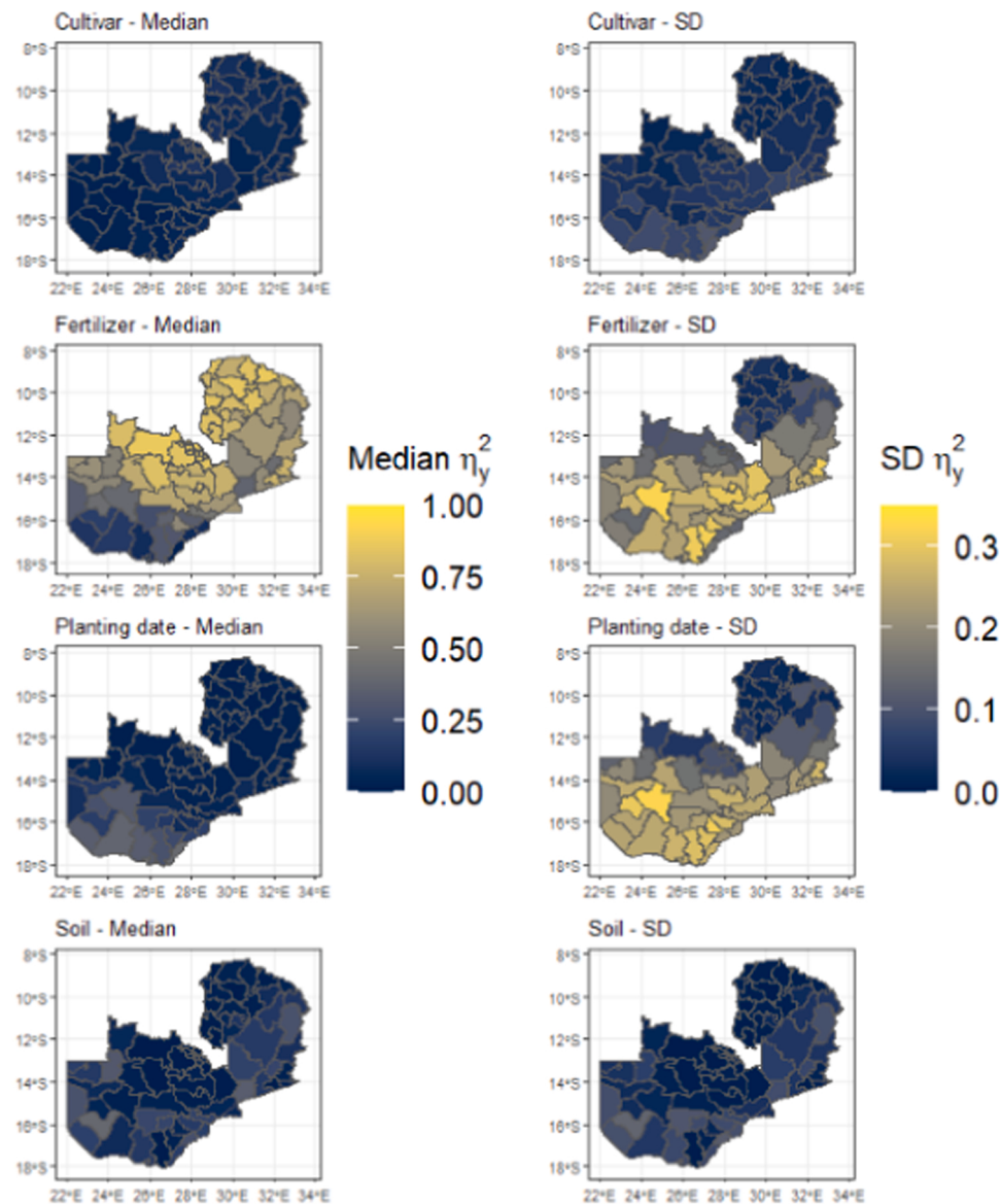
Fig. 7. Median (left) and standard deviation (right) of yearly effect sizes ( \eta_y^2 ).
