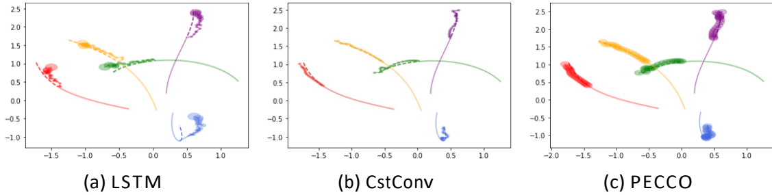
Figure 3: Comparison of prediction results between baselines. The solid lines are input timesteps to the models, the dotted lines ground truth, and the circles the 90% confidence regions. We can see that PECCO achieves accurate results while maintaining good coverage.
