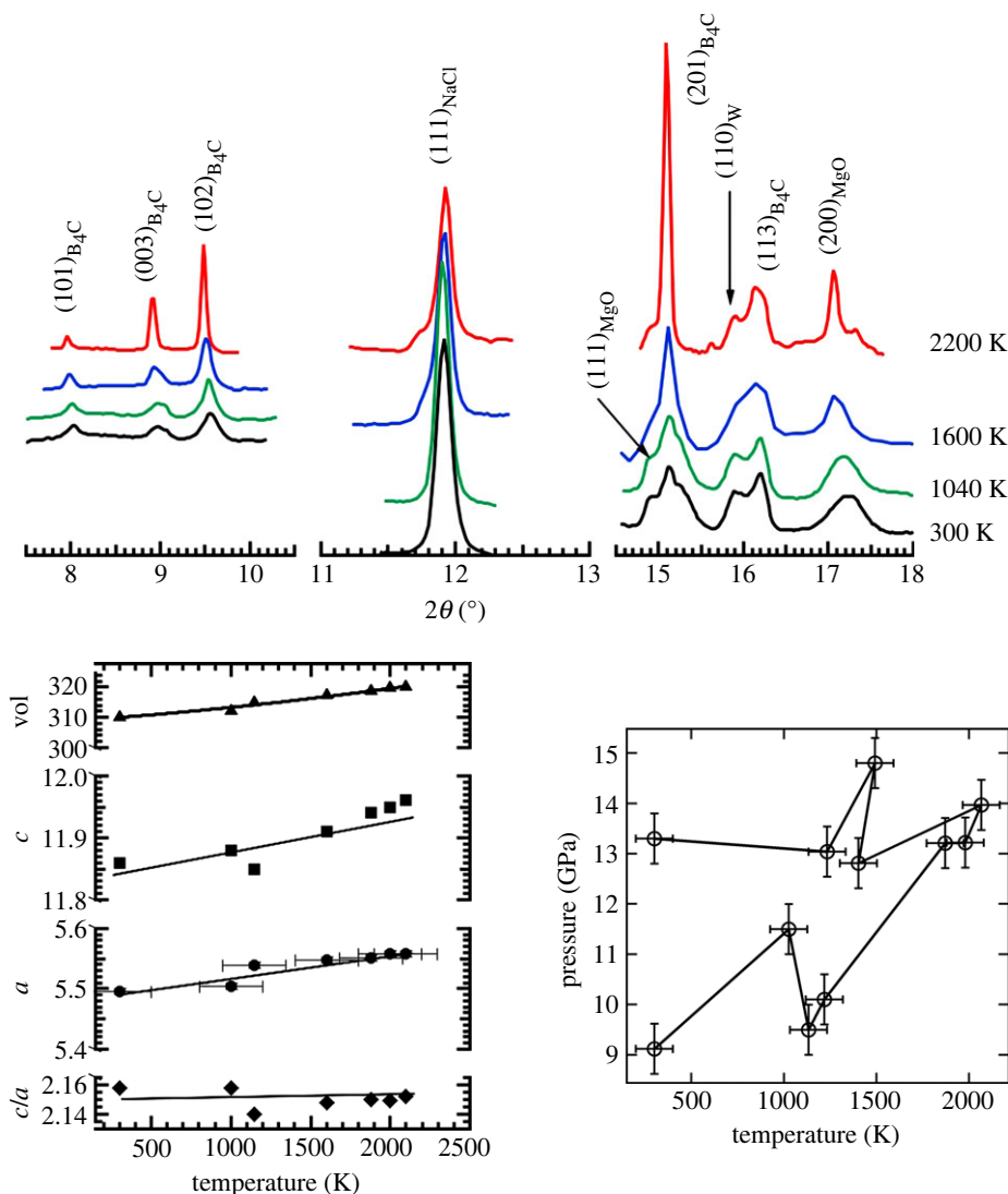
Figure 2. The top panel shows representative X-ray diffraction patterns obtained at a starting pressure of 9.1 GPa and subsequent laser heating. The diffraction peaks (111)_{\text{MgO}} and (200)_{\text{MgO}} were used to obtain the unit cell volume of MgO. The resulting pressures obtained from MgO P-V-T EOS [13] at various temperatures are plotted in the lower right panel and the cell constants of \text{B}_4\text{C} obtained in the lower left panel. The error bars in pressure are estimated from the width of the MgO diffraction peaks while the error bars in temperature are deduced from the overall drift in temperature and the imbalance between the two sides (upstream and downstream heating spots). Since this was the first heating cycle, there was considerable drift in sample pressure. Subsequent heating at higher starting pressures did not show this large a drift and typically remained within approximately 2 GPa. (Online version in colour.)
