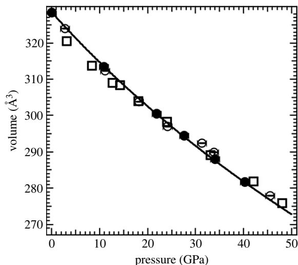
Figure 1. Pressure–volume data of B_4C obtained from two different runs together with the fit to a second-order Birch–Murnaghan equation of state (solid line, V_0 = 328.5 \text{ Å}^3 , K_0 = 221 \text{ GPa} and dK_0/dP = 3.3 ). The filled circles correspond to results from samples quenched from above 2000 K to ambient temperature which were used to constrain the fit. The empty circles represent the ambient data obtained without any thermal annealing. Both the filled and empty circles represent data obtained from an NaCl medium with MgO as pressure standard. The error bars in pressure represent the difference between pressure estimated from NaCl and MgO [13] diffraction data. Superposed are the P–V data obtained with a neon pressure medium where the pressure was determined using ruby fluorescence (empty squares).
