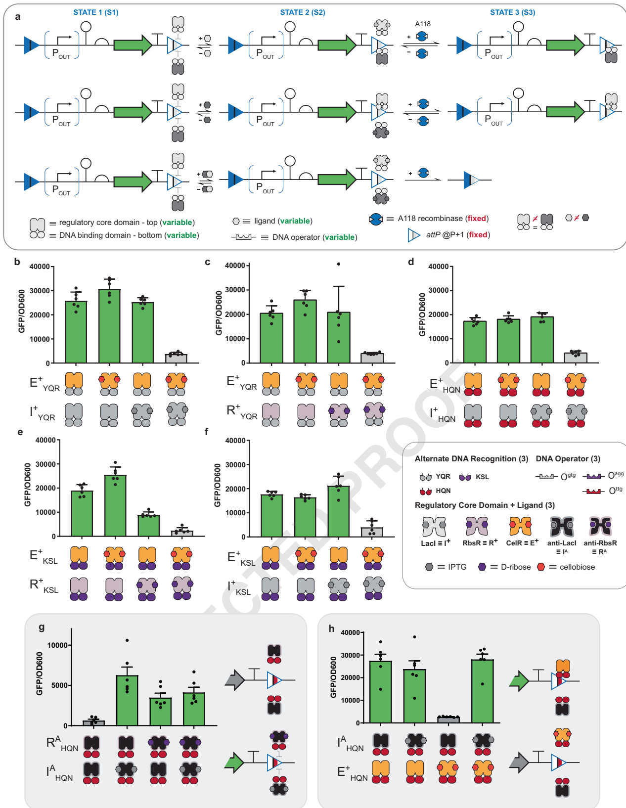
Fig. 6 | Multiple input interception memory. a Schematic of interception of a deletion circuit by two transcription factors (TFs). The regulatory core domains and DNA-binding domains vary, and corresponding ligands and DNA operators are used in each case. A118 recombinase is constitutively expressed in all cases, and the variable operators are always placed at the P + 1 position. The state diagram presents the relationship between repressor, ligand, operator, and recombinase with each set of ligands added. b–f Interception with two repressors. b E + YQR and I + YQR
