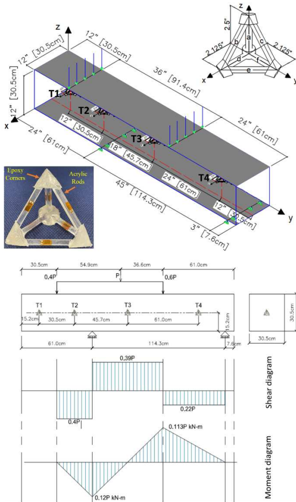
Fig. 1. The prototype tetrahedron sensor, the validation beam test setup, and shear and moment diagrams
