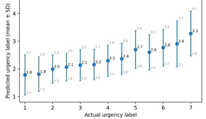
Figure 1: Prediction results of the best performing model (SVR) on the separate test set using the word count features.
