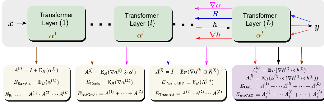
Figure 2: A summary of the existing explanation methods and our methods: CAT and AttCAT. The Transformer consists of several layers denoted as Layer (1), ..., (l), ..., (L). \nabla \alpha and \nabla h represent the gradients of attention weights \alpha and outputs h , respectively. R is calculated based on layer-wise relevance propagation (LRP). \mathbb{E} denotes the explanation method. \mathbb{E}_H means averaging among multi-head attentions in each layer.
