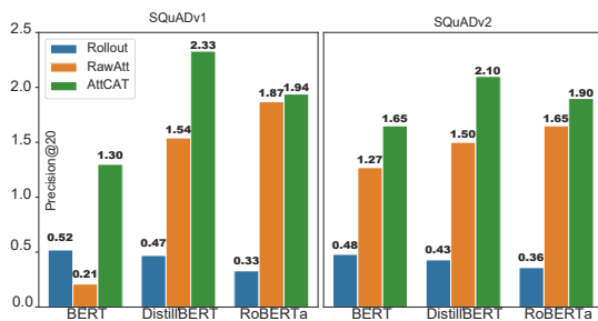
Figure 4: Precision@20 scores of the selected explanation methods for different Transformer models on SQuAD data sets. Higher scores are better. The Rollout on SQuAD data sets. Higher scores are better. The and Sum denote the rollout and summation max scores of SQuADv1 and SQuADv2 are 3.72 operations (ours), respectively. Best viewed in and color.
